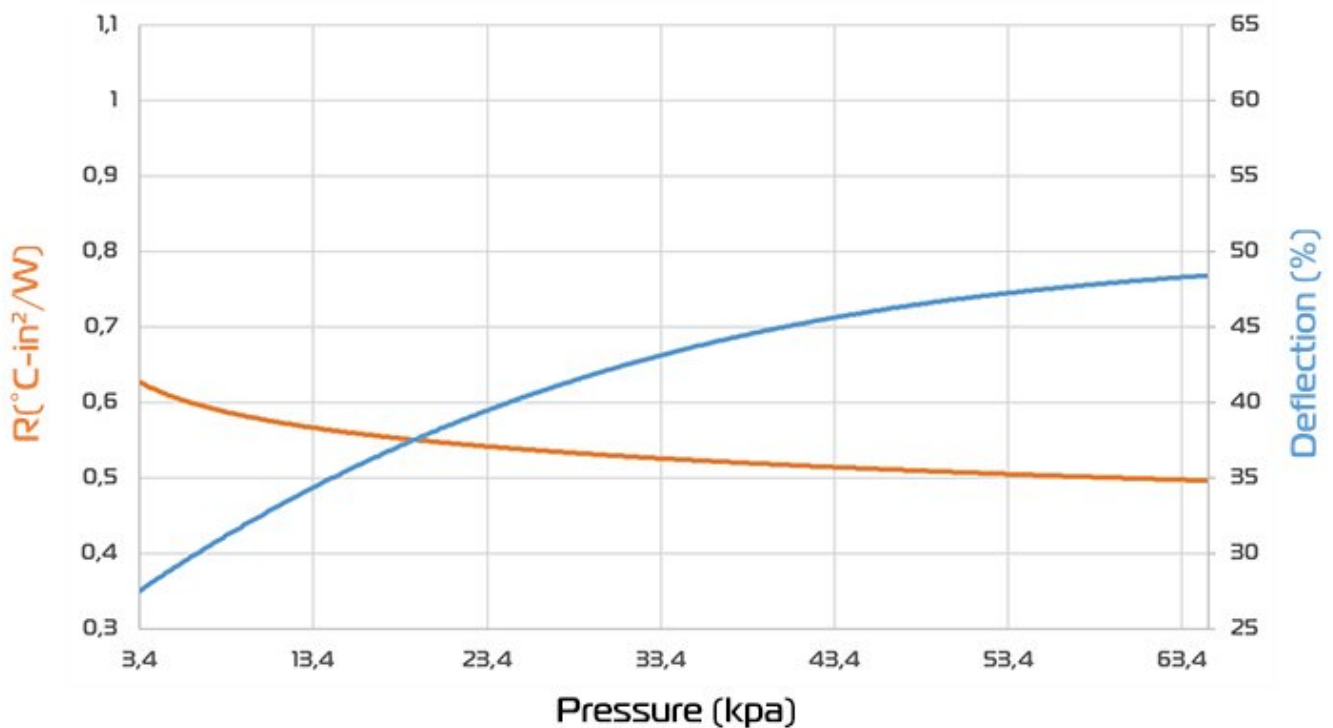
Thermal Resistance vs. Pressure vs. Deflection
