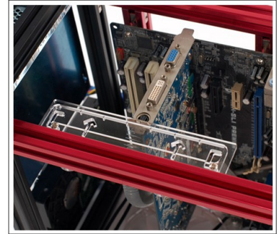
ATX Seven Slots PCI fixed block is fixed on the outside of aluminum profile
