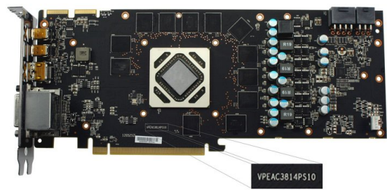
XFx Radeon HD 7970/7950 Custom PCB
