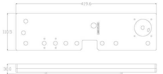
RGV-TT-P3 FRONT VIEW, SIDE VIEW Dimension In"MM"
