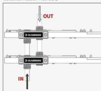
Dual Graphics card inlet and outlet connection method 3
