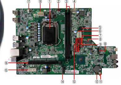
Main-board Placement
