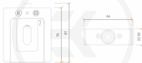
TOP VIEW, SIDE VIEW
